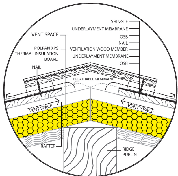
DETAIL A ALTERNATIVE 2 IN-SITU FABRICATION
