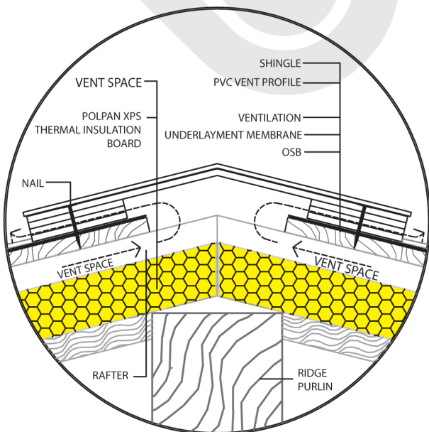
DETAIL A ALTERNATIVE 1 VENT PROFILE
